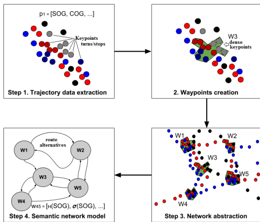
Figure 2: The main steps of the proposed model.
